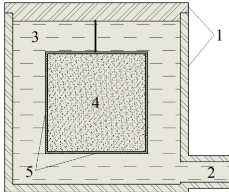
Fig. 1. the working chamber of the hydrostat: 1 – pressure-tight chamber, 2 - fluid input, 3 - working fluid, 4 - powder, 5 - elastic shell
